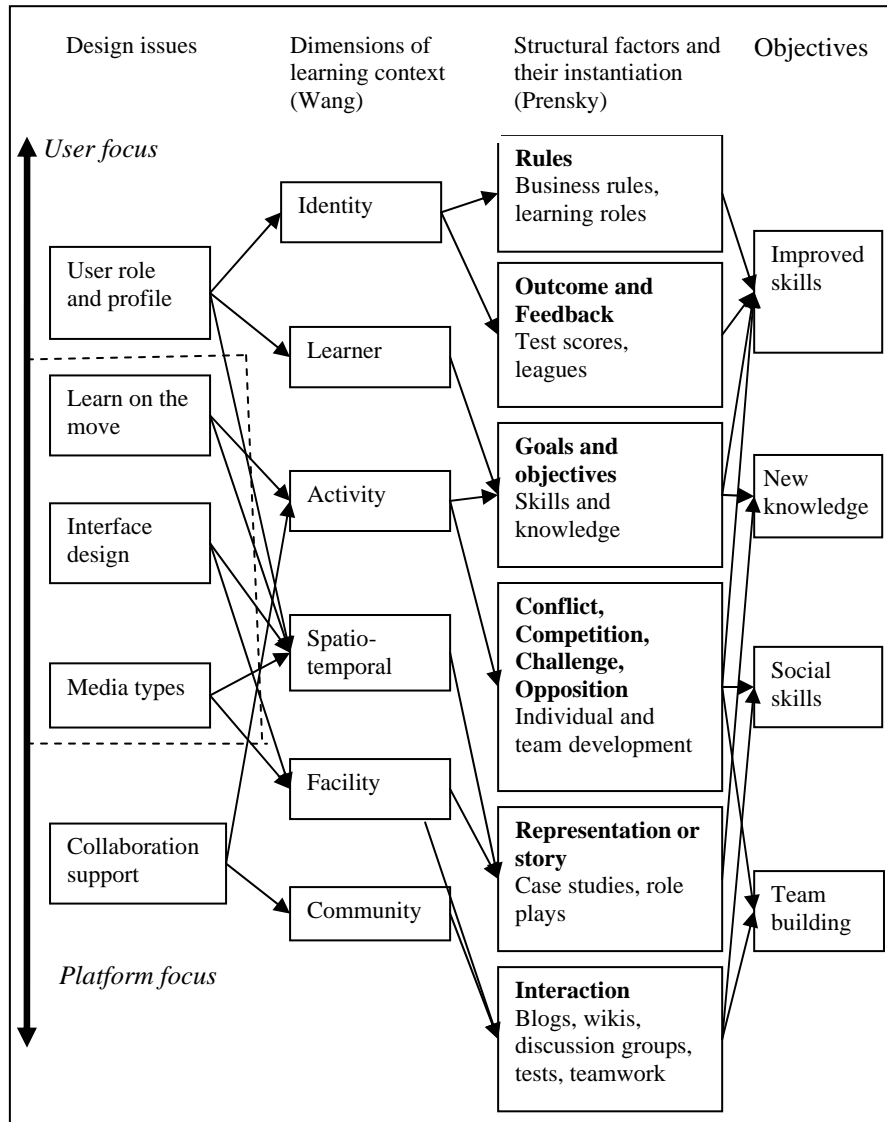
Figure 1: A conceptual design framework for M-learning
