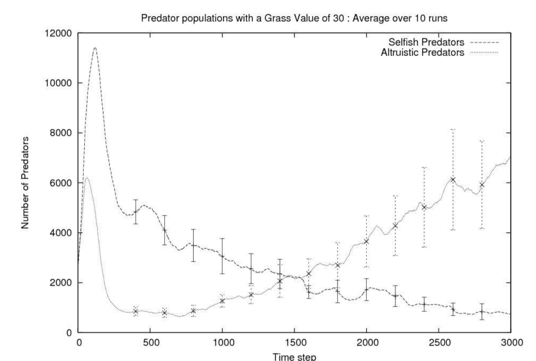
Figure 4: Time evolution of selfish and altruistic predators over a typical model run.
