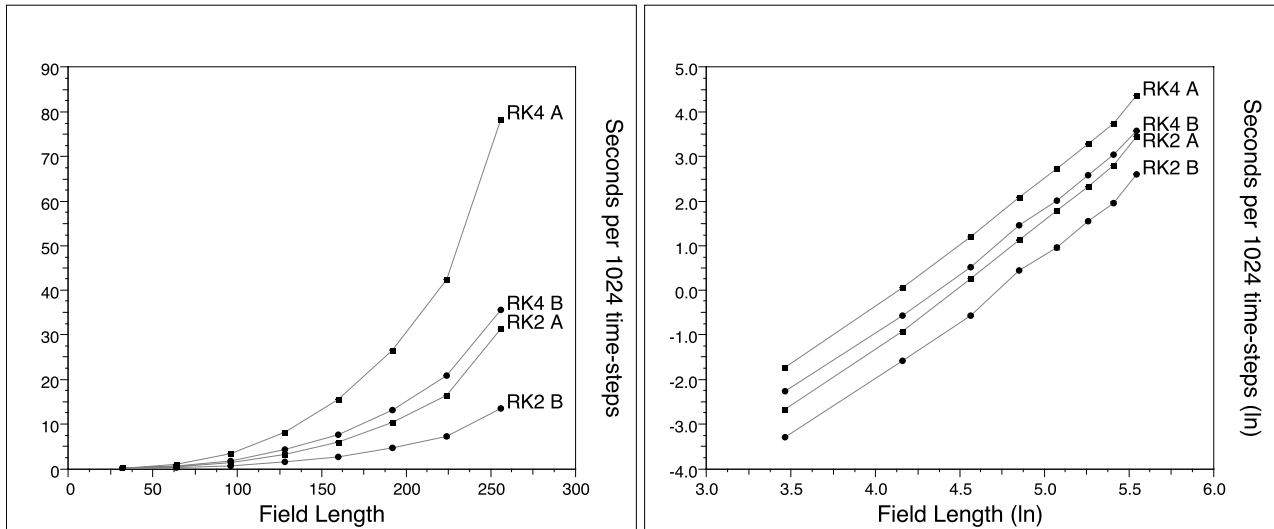
Figure 4: A comparison of the CUDA implementations A&B across field lengths N = \{32^3 \dots 256^3\} . Note that the error in the timing is not shown as the error bars are smaller than the symbol size of the plots. Results are shown in normal scale (left) and ln-ln scale (right).
