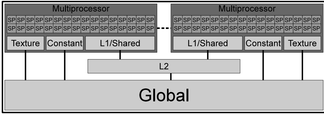
Figure 3: The architecture of NVIDIA Fermi GPUs.
