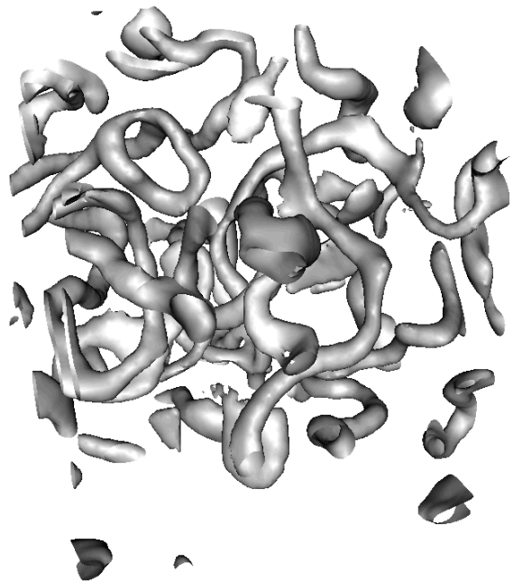
Figure 1: A iso-surface map of the magnitude of a simulated Ginzburg-Landau Field showing helical vortices and other spatial structure in the order parameter.
