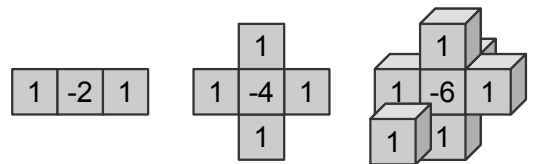
Figure 2: Laplacian operator in one-, two- and three-dimensions.
