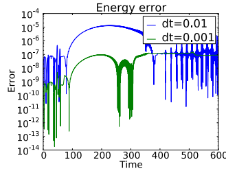
FIG. 5.2. The energy error over time. This is the energy at each step minus the initial energy. The bicycle is trapped in the potential bowl -V(\mathbf{q}) , and the energy error does not show a linear growth in time.
