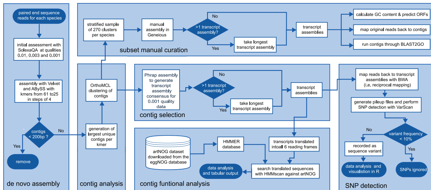
Fig 2. Bioinformatic pipeline for analysis of cDNA from non-model organisms with large polyploid genomes to test hybrid origin hypotheses.
