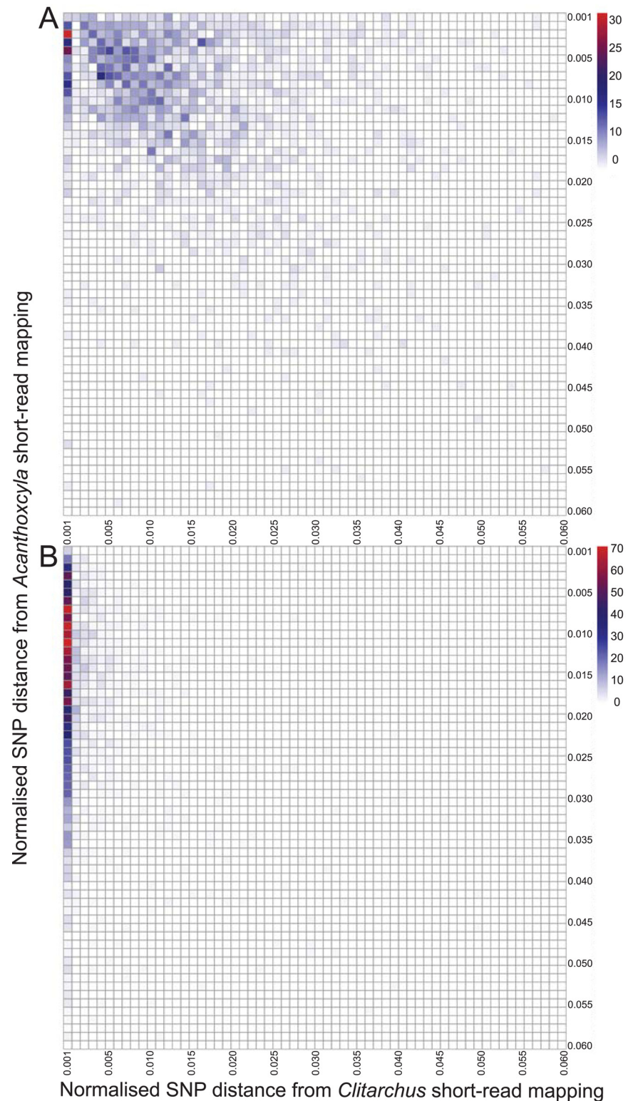
Fig 4. A similar level of genetic divergence within a hybrid stick insect genome as is observed between parental alleles when alleles are compared. Heat maps of sequence similarity between short-read cDNA sequences mapped to transcript assemblies. (A) Acanthoxyla transcript assemblies with
