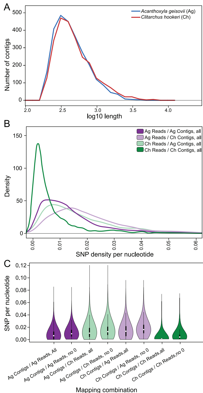
Fig 3. Next Generation sequencing results from mRNA of two New Zealand stick insects (A). Length distributions of transcript assemblies produced from the cDNA sequence of two stick insects were similar. A log length frequency distribution plot used values rounded to 1 decimal place for the longest consensus
