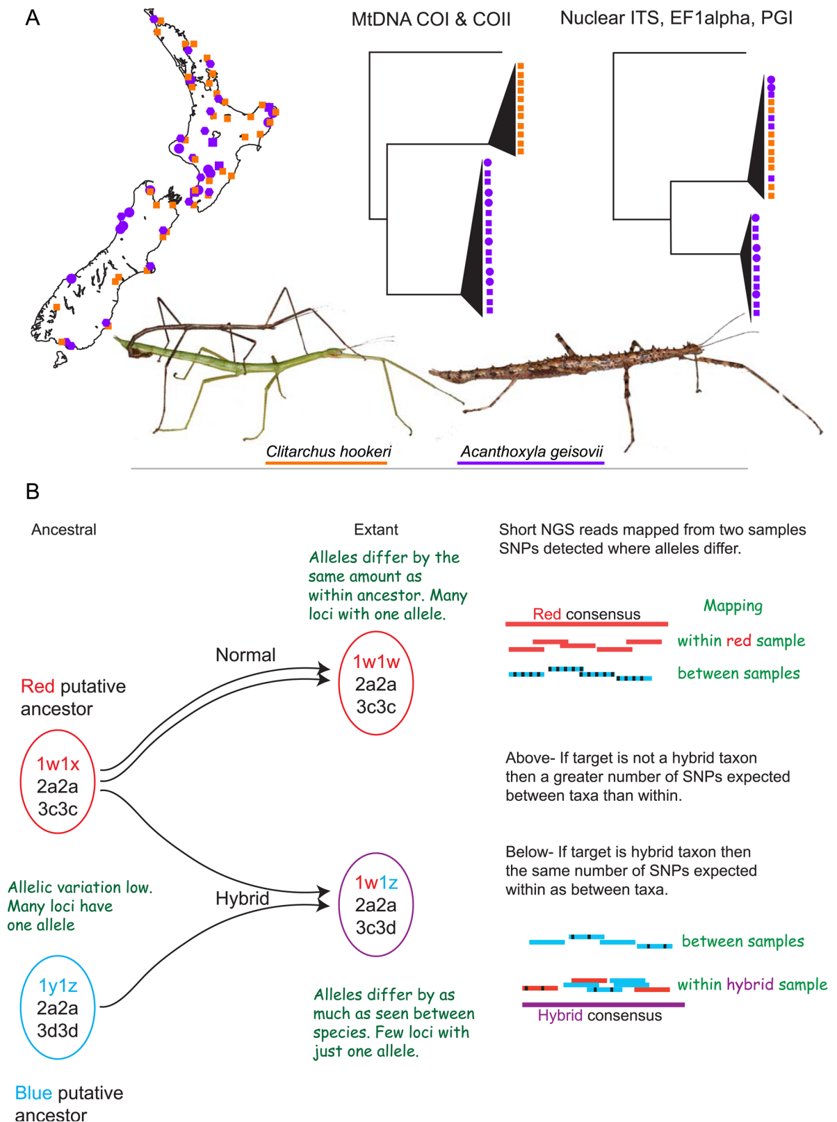
Fig 1. New Zealand stick insects illustrate hybrid speciation hypotheses that arise from evolutionary studies. (A) Two lineages of stick insects have been sampled across their range in New Zealand and by contrasting maternal relationships from mitochondrial DNA sequences with bi-parental multicopy nuclear markers a role for hybridisation has been inferred. Diploid
